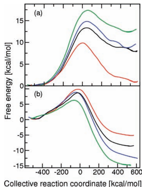
Figure 2. Potential of mean force (PMF) curves for (a) the first proton transfer step and (b) the second proton transfer step catalyzed by KSI. These profiles are depicted for the WT (red), D99L mutant (black), Y14F mutant (blue), and Y14F/D99L double mutant (green) forms of KSI. For both steps, all curves are shifted so that the reactant is at zero energy, although mechanistically the product of the first step is the same as the reactant of the second step, following rotation of the Asp38 carboxylate group.
