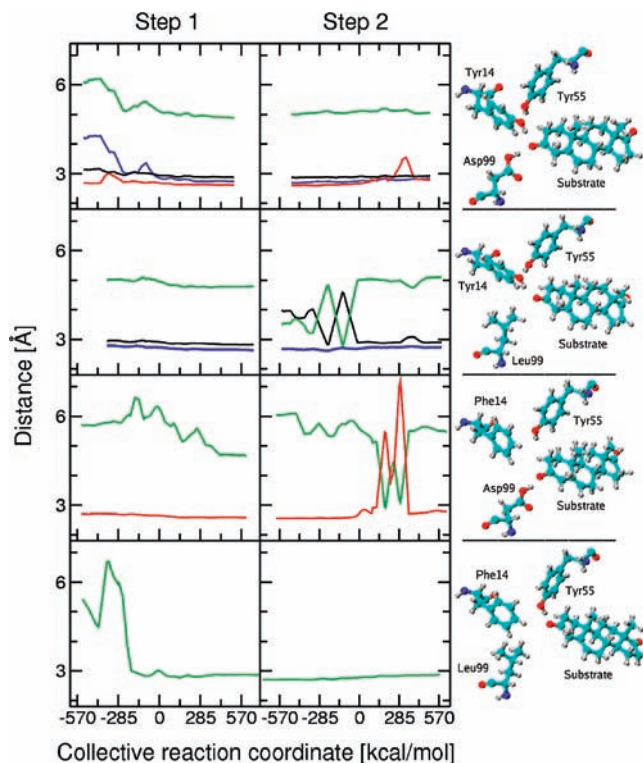
Figure 4. Thermally averaged distances calculated along the collective reaction coordinate for the first (left) and second (right) proton transfer reactions catalyzed by KSI. Snapshots of the hydrogen-bonding pattern in the active site for the Intermediate state are also depicted. The results for the WT, D99L, Y14F, and Y14F/D99L mutants are given from top to bottom. The thermally averaged hydrogen bond donor–acceptor distances between the substrate O3 atom and Tyr14 (blue), between the substrate O3 atom and Asp99 (red), between the substrate O3 atom and Tyr55 (green), and between Tyr14 and Tyr55 (black) are shown. All distances shown are between the two oxygen atoms in the hydrogen bond. The distances are not shown for the mutated residue. The color coding is depicted in Figure 3.
